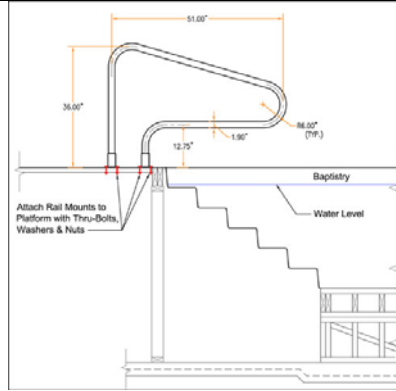
Hand Rail
